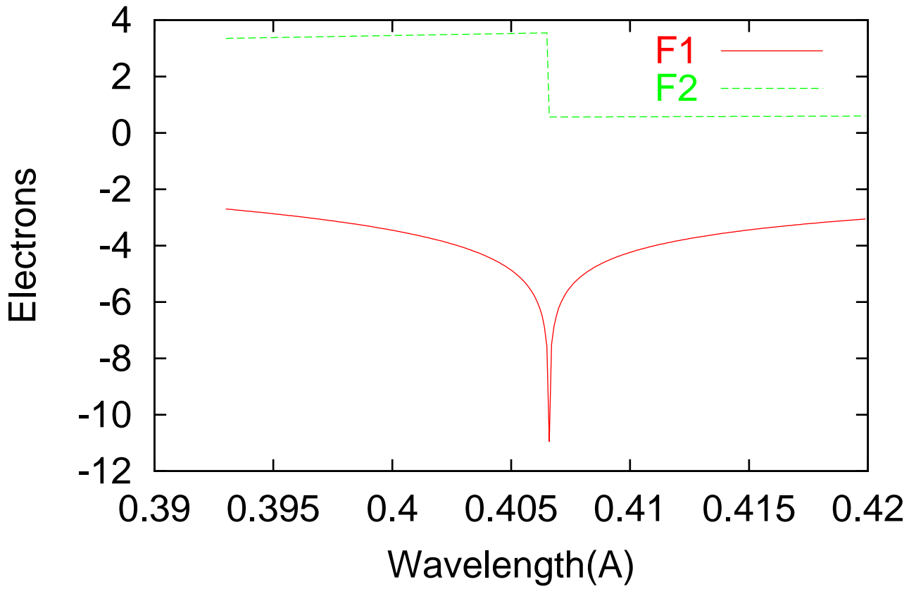
Absorption Data ( SB.K )
